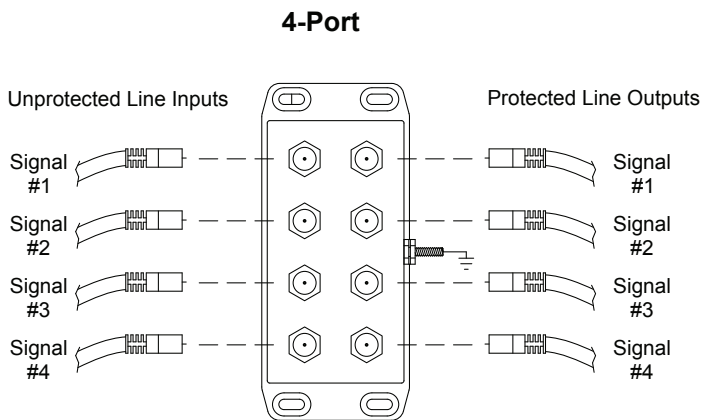
Fig. A - CONNECTION METHOD
