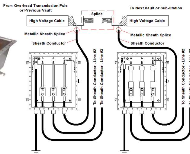
TLb-GND Series Link Box with Ground Bars
